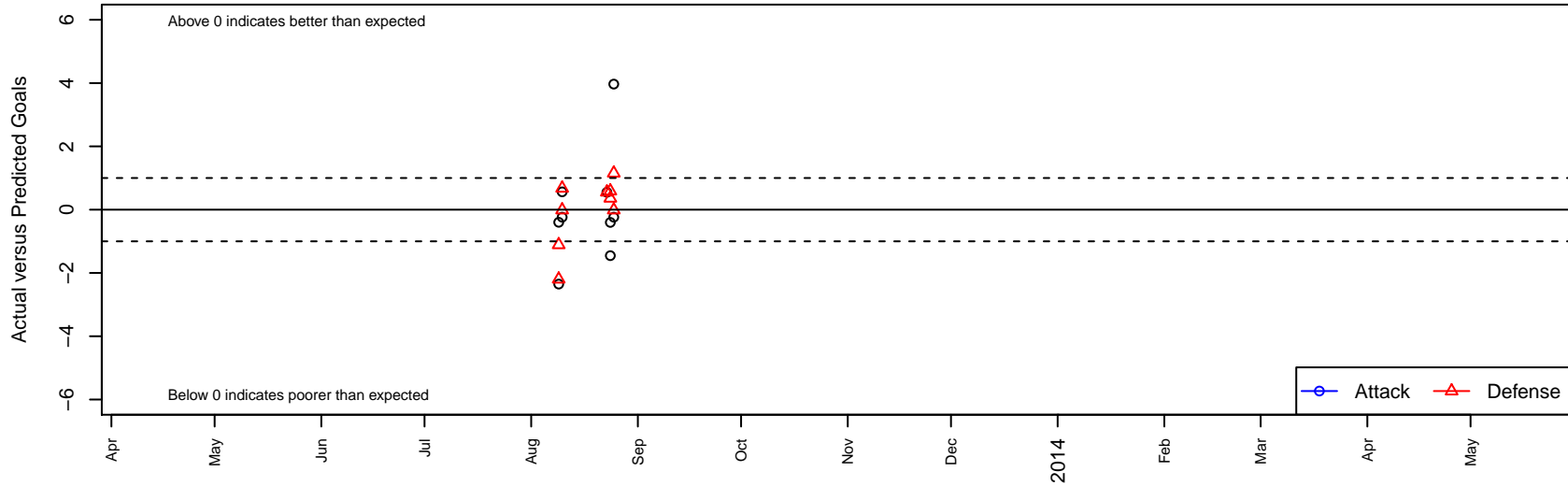
San Jose Earthquakes East Valley B00 Dots are actual minus expected GF (blue circles) and GA (red triangles). Blue line is smoothed change in attack strength. Red is smoothed change in defense strength.
